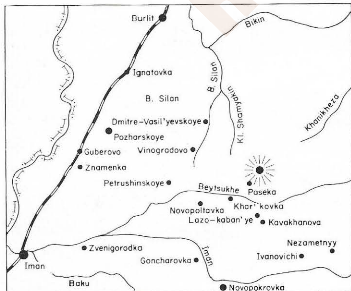
To right of center on this map, radial lines indicate the meteorite fall. Iman and Burlit are on the Trans-Siberian railroad. At right is V. G. Fesenkov's orbit of the parent body in the solar system.
