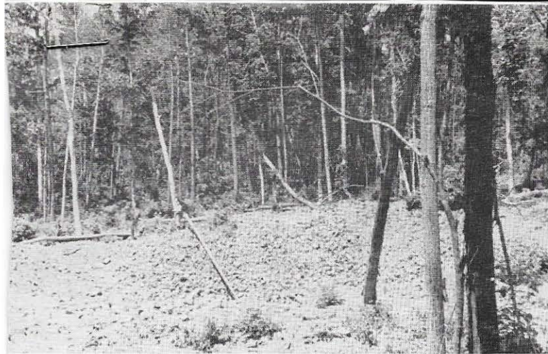
In 1948, when the second expedition investigated the great Sikhote-Alin meteorite fall, the largest crater appeared as at left. It was 26 meters wide and six meters deep. But after two decades, vegetation almost hides the crater from view (right). This picture was taken by the expedition led by E. L. Krinov during the summer and fall of 1967. Unless otherwise credited, illustrations with this article are from the author, courtesy Novosti Press Agency.
