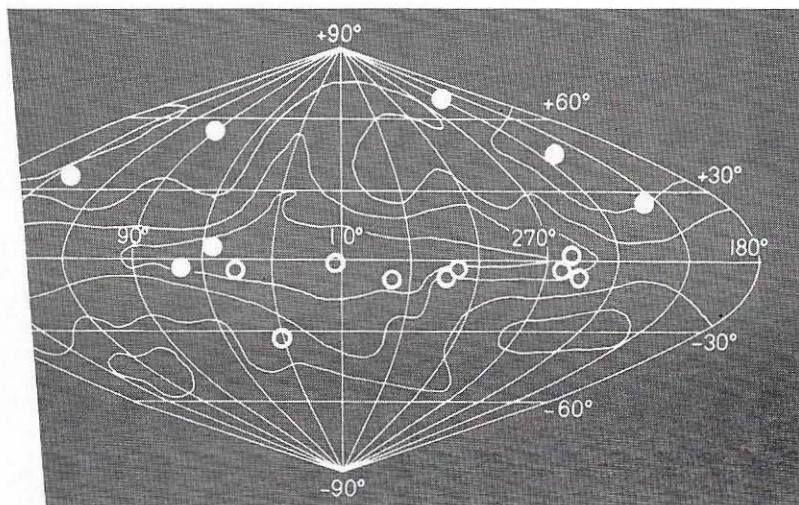
Pulsars are plotted here on a grid of galactic coordinates (Milky Way longitude and latitude), with Molonglo Radio Observatory discoveries as open circles. Radio wavelength background isophotes from radio observations are shown. Cornell-Sydney universities diagram, from Nature .
