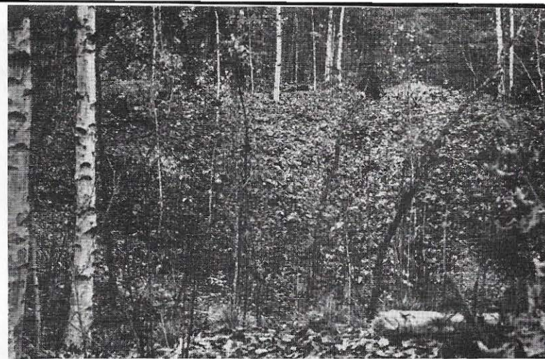
In 1948, when the second expedition investigated the great Sikhote-Alin meteorite fall, the largest crater appeared as at left. It was 26 meters wide and six meters deep. But after two decades, vegetation almost hides the crater from view (right). This picture was taken by the expedition led by E. L. Krinov during the summer and fall of 1967. Unless otherwise credited, illustrations with this article are from the author, courtesy Novosti Press Agency.
