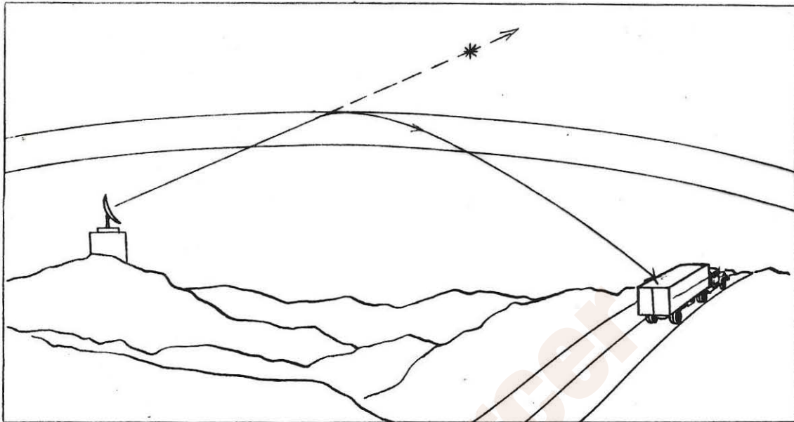
Figure 3 Inversion layer causes the radar beam to bend and pick up the truck on the highway giving the appearance of a high slow-moving target.
