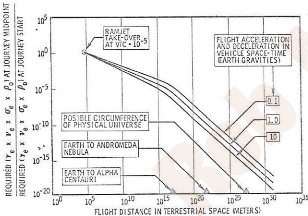
Figure 4 - Vehicle and Fuel Demands
