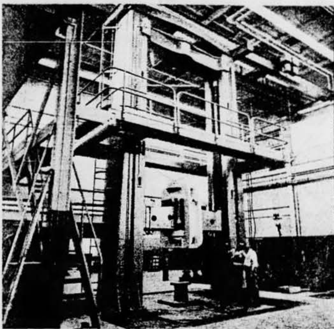
A feature of the Center is the 1,000,000 pound static testing machine, with the largest testing clearance of any million-pound machine yet built.
