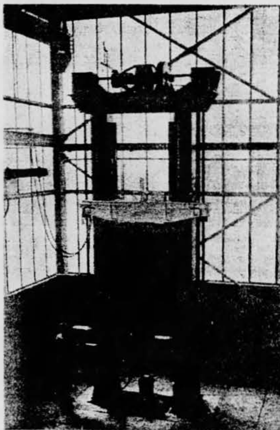
The 27,000 pound drop test machine is mounted on a 500,000 pound concrete-and-steel inertia block. Shock isolation is provided in the foundation.
