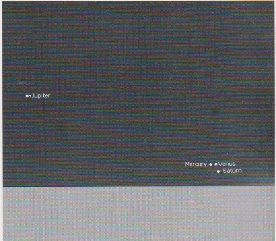
Conjunction of Mercury Venus and Saturn
