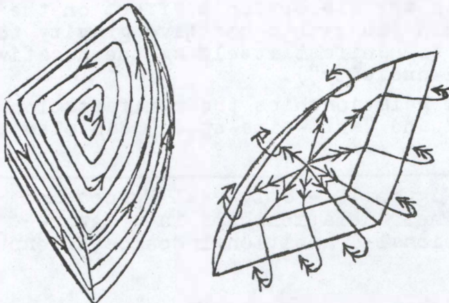
Spiral Cone Coil (from top) Resultant magnetic field (from bottom)
