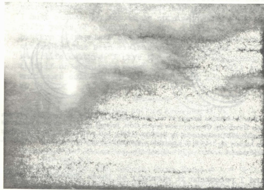
FIG. 6—A subsun, seen on a flight over Europe in November, 1966. (Photo by Author)
