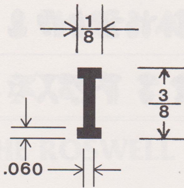
I-beam dimensions.
